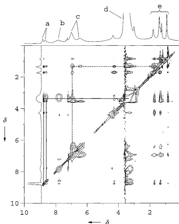
Figure 3. NOESY MAS NMR spectrum of porphyrin-stoppered rotaxane 3 showing NOE cross-peaks between the PEG chain and the outer aromatic protons of 1 (solid line), and between the polystyrene backbone of the ArgoGel and the pentyl side chain of 1 (dotted line). The 1D spectrum shown on the F2 axis is the 1 H MAS NMR spectrum of 3 , and the 1D spectrum shown inside the box is a cross-section taken from the NOESY experiment at \delta = 8.87 . Resonances a correspond to the inequivalent outer aromatic protons of 1 (see text), and resonances b, c, d, and e correspond to the other aromatic protons of 1 , the polystyrene backbone of ArgoGel, PEG, and the pentyl side chains of 1 , respectively.
